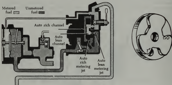
FIGURE 3-26. Manual mixture control, auto-lean setting.
